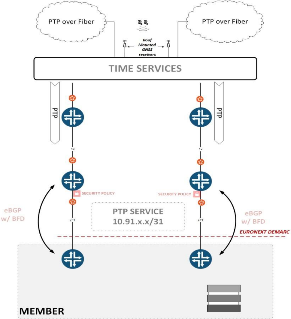
Figure 1 - Schematic of equipment set-up for PTP time source and PTP Feed Distribution
